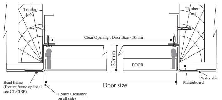
Bead Frame in single layer Joist plasterboard application
