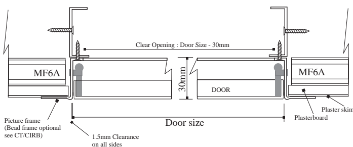
Bead Frame in single layer MF plasterboard application
