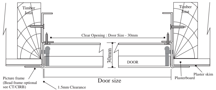
Picture Frame in single layer Joist plasterboard application
