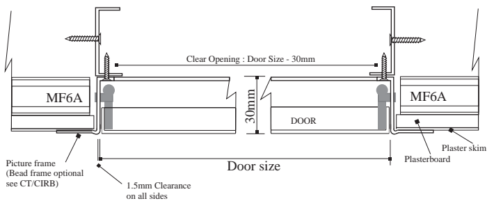
Bead Frame in single layer MF plasterboard application
