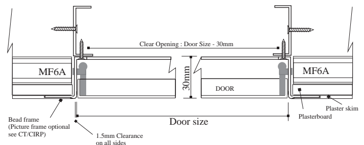
Bead Frame in single layer Joist plasterboard application
