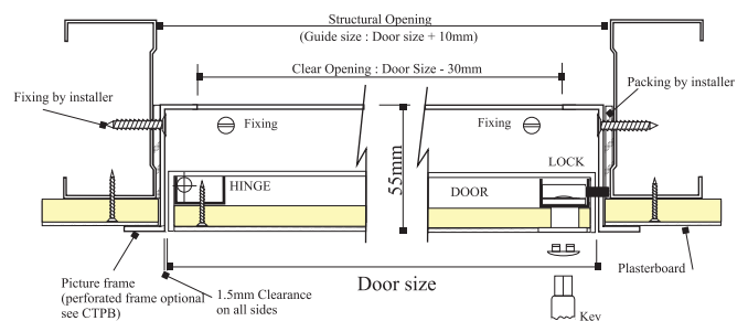
Single layer plasterboard application (NFR)
